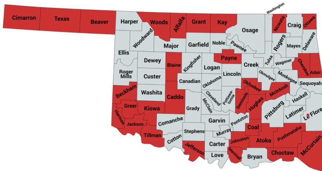
Figure 2: Non-metro Oklahoma counties with at least one stressor
